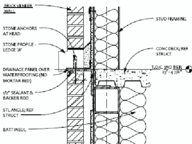
2 SECTION - FLUSH TOWER LEDGE @ SLAB 1 1/2" = 1'-0"
